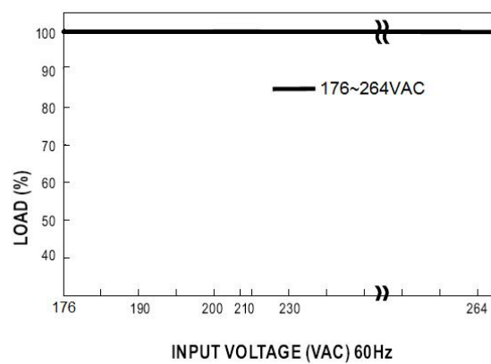
■ Static Characteristics
